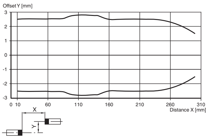
Characteristic response curve High Precision Modus
