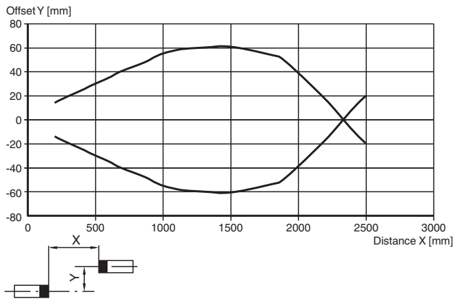
Relative received light strength Long Range Modus
