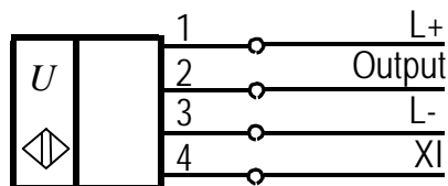
3RG6342-3AA00-PF:
