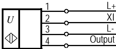
3RG6342-3AB00-PF:
