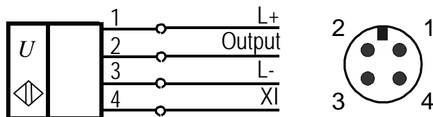
3RG6343-3AA00-PF:
